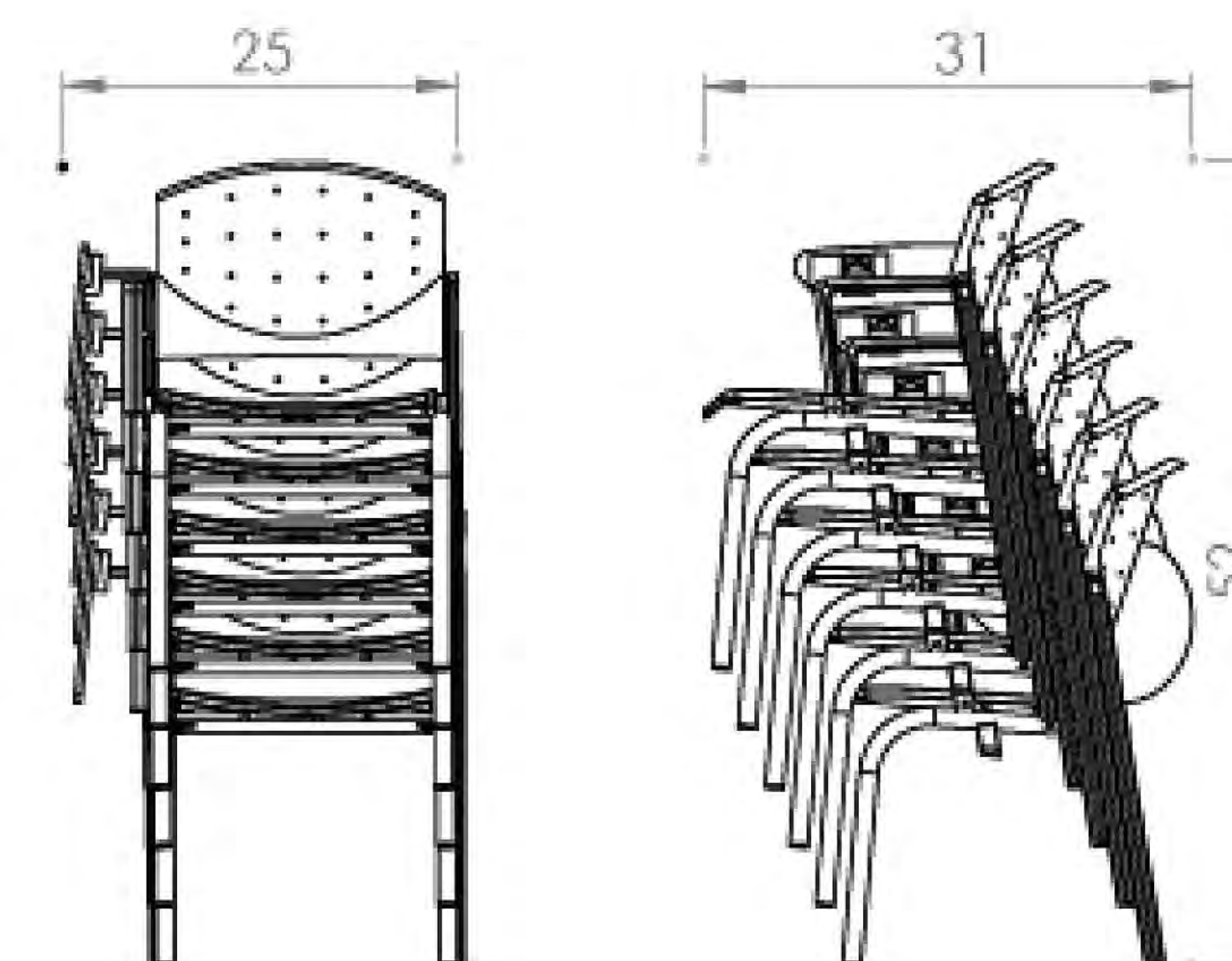
EDDY 4-POST WITH TABLET | Stacks 6 on Floor
