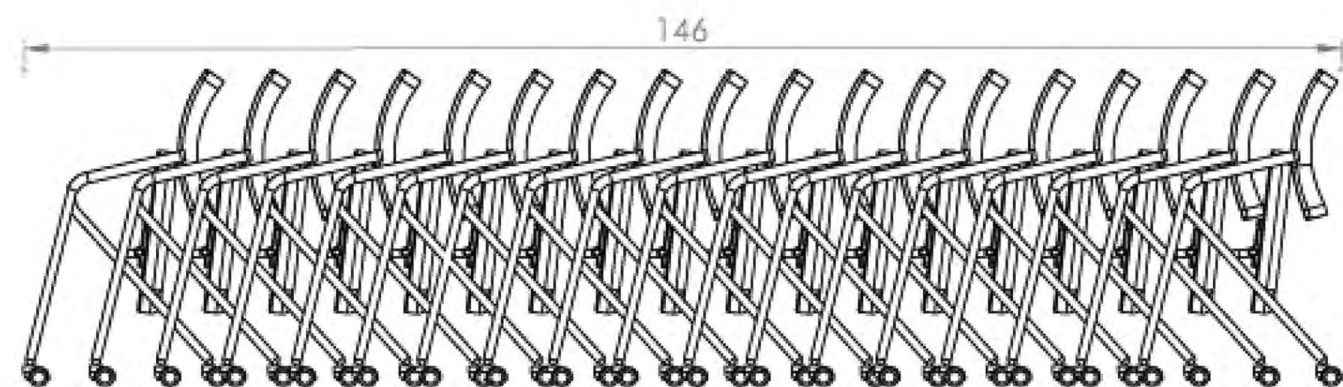
JOIN ME | Nesting 18 Chairs
