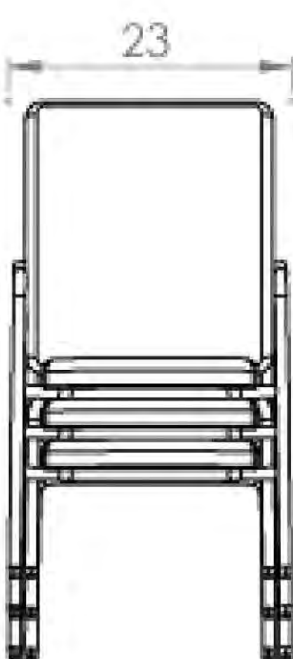
LOGAN 4-POST | Stacks 3 on Floor
