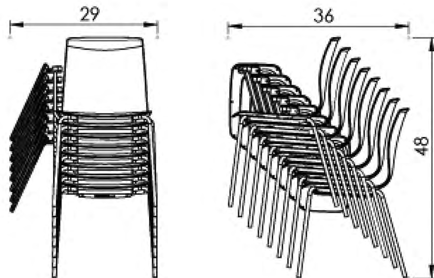
CEMPA 4-POST WITH TABLET | Stacks 8 on Floor
