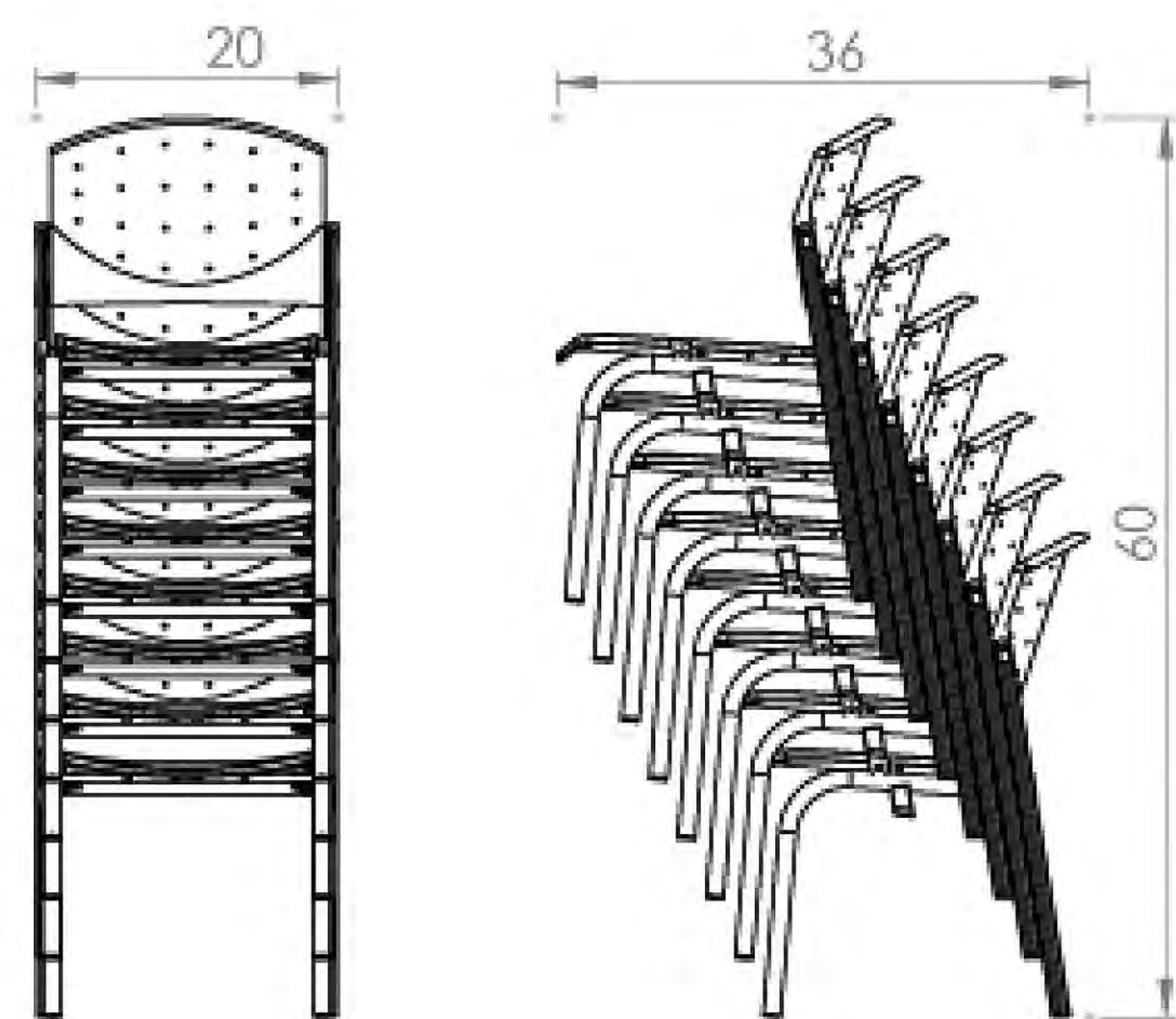
EDDY 4-POST | Stacks 8 on Floor
